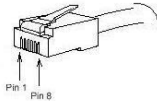
Figure 3-6 RJ-45 connector of the console port
