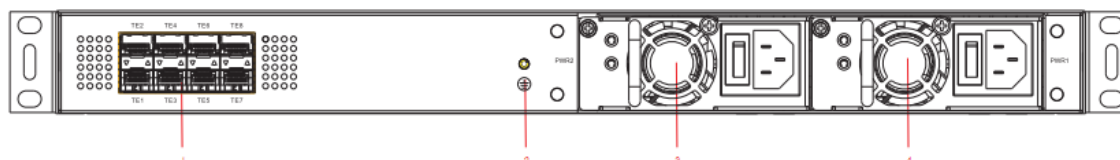
Figure 1-2 The back template of the S3756P switch
