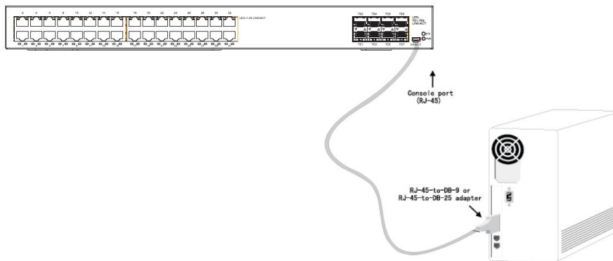
Figure 3-5 Connecting the console port of S3740 and computer
