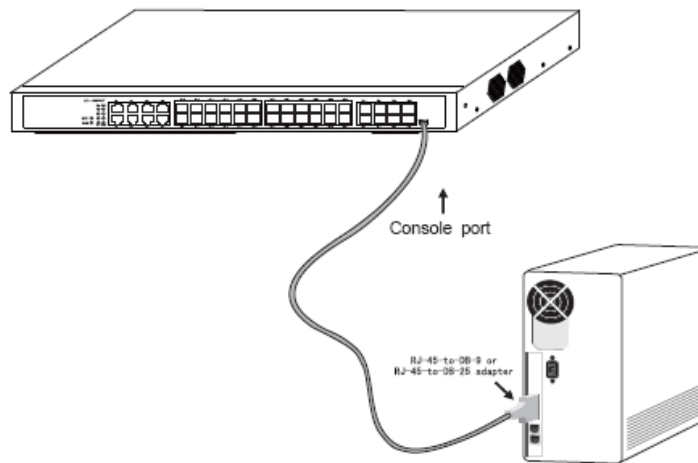
Figure 3-5 Connecting the console port of S3740F and computer
