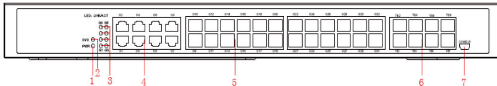
Figure 1-1 Front template of the S3740F switch
