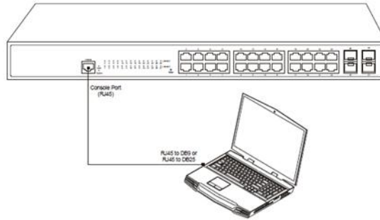
Figure 3-4: Connecting the console port of S2528-B with the computer
