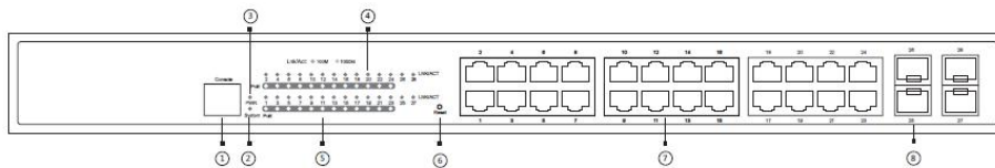
Figure 1-1 Front template of the S2528-B switch
