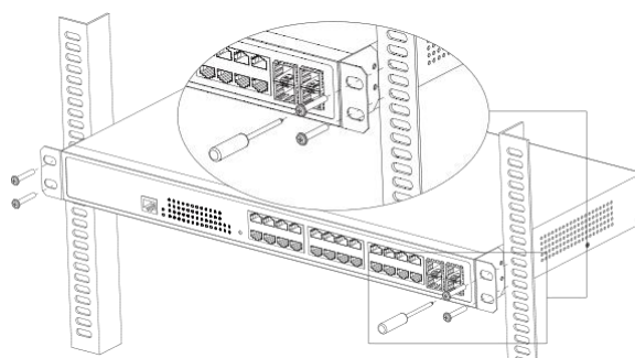
Figure 3-2: Installing the switch on the cabinet
